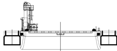
FRONTVIEW HEBO P41/P42 COUPLED
