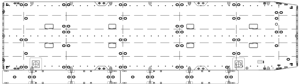
TOPVIEW HEBO P41/P42 COUPLED OPTION 2
