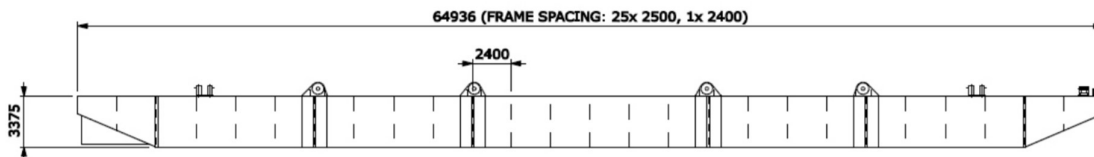
Side view
